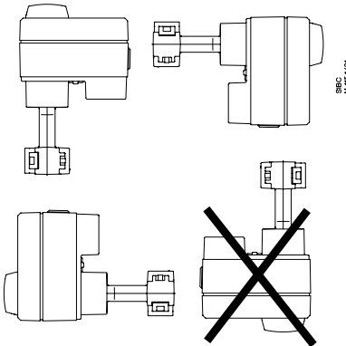
AMV(E) 15 VL2/VL3 DN 15 - 50 mm
