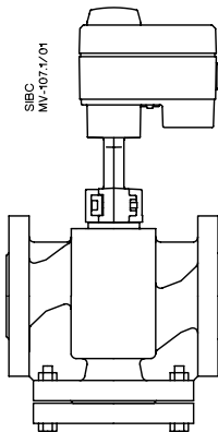
AMV(E) 15 VL2/VL3 DN 15 - 50 mm
